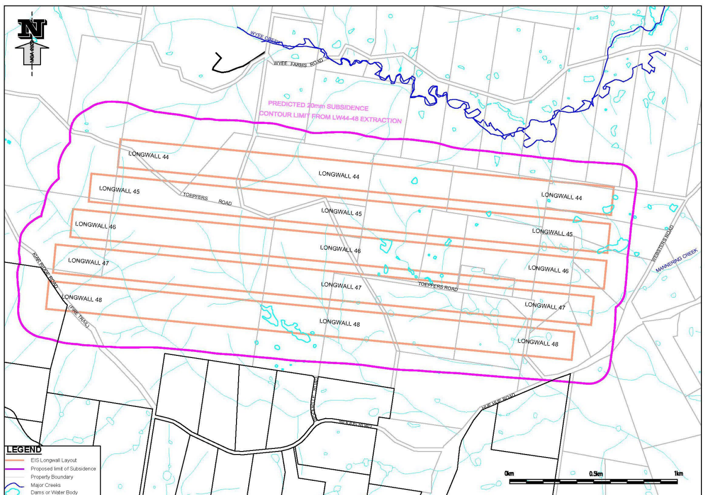
Figure 2: Mandalong mine plan for Longwalls 44 to 48.
